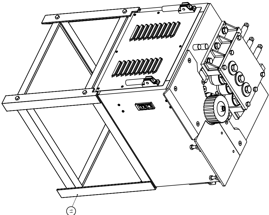
FRONT ISOMETRIC VIEW
